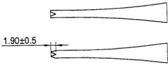
DETAIL 1 x 2 TEETH SCALE 1:1
