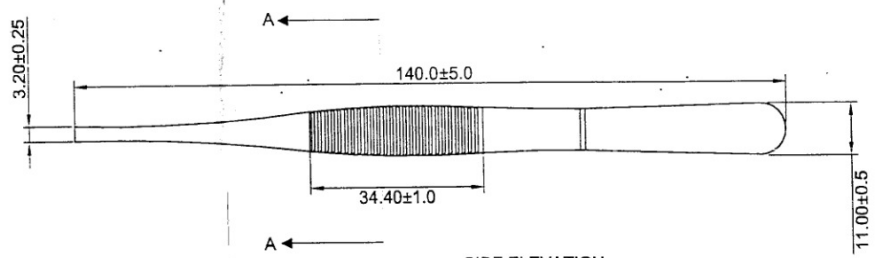
SIDE ELEVATION
